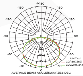
· Photometric of 1M strip
